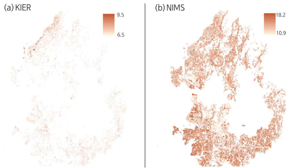
Fig. 1. Market potential of PV: KIER vs. NIMS (MWh/year/100m²)
